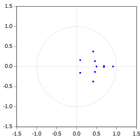
Figure 1. Inverse Roots of the Characteristic Polynomial for the Regression Model
